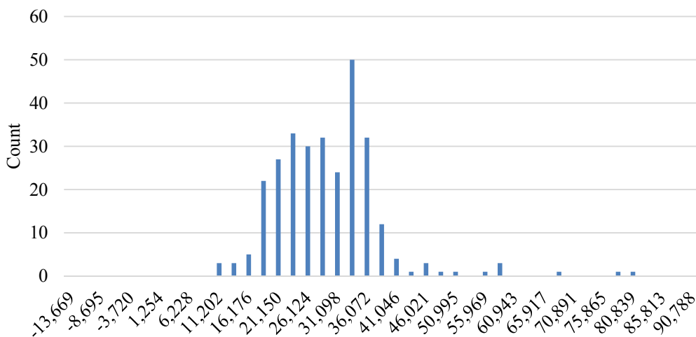
Figure 1 - Pretransition Costs Histogram
