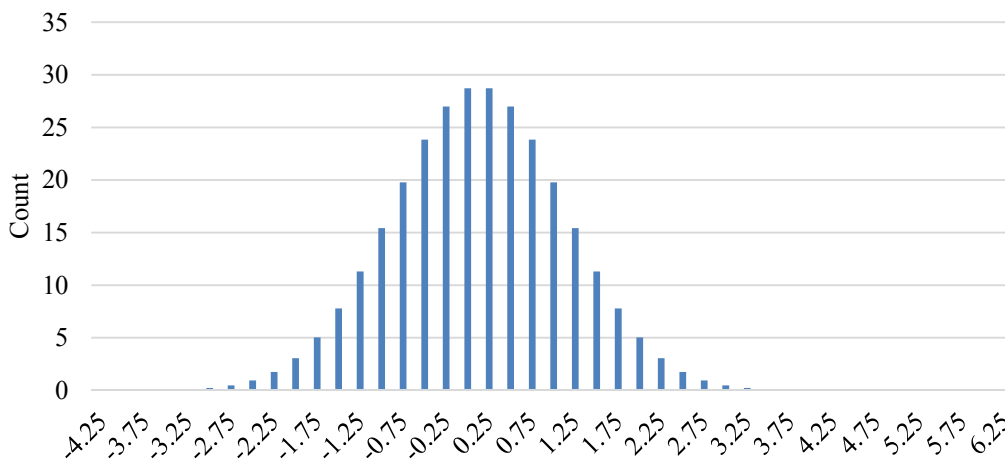
Figure 4 - Normal Distribution Histogram
