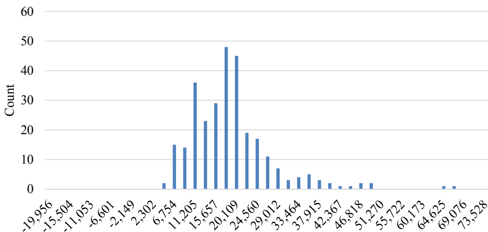
Figure 2 - Post Transition Costs Histogram
